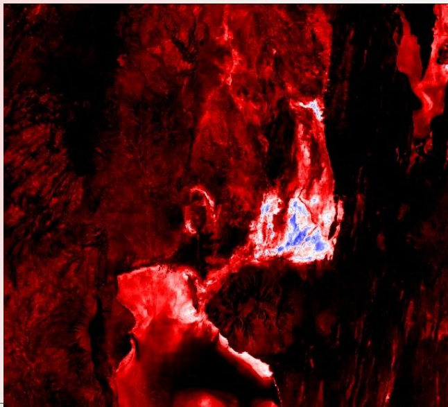
Cosine Similarity
