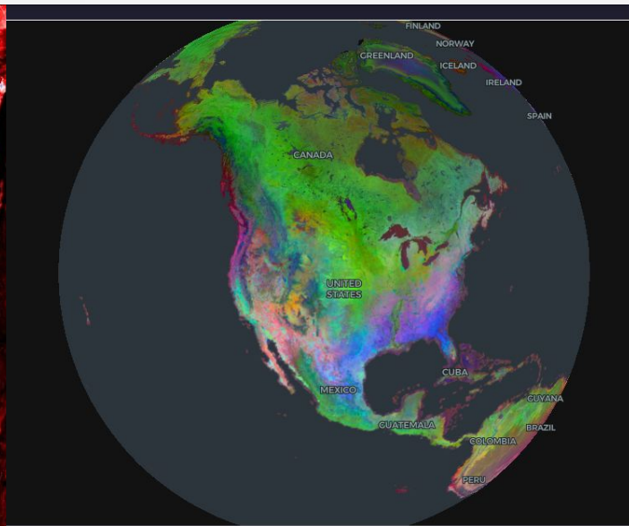
False-Color Imagery
