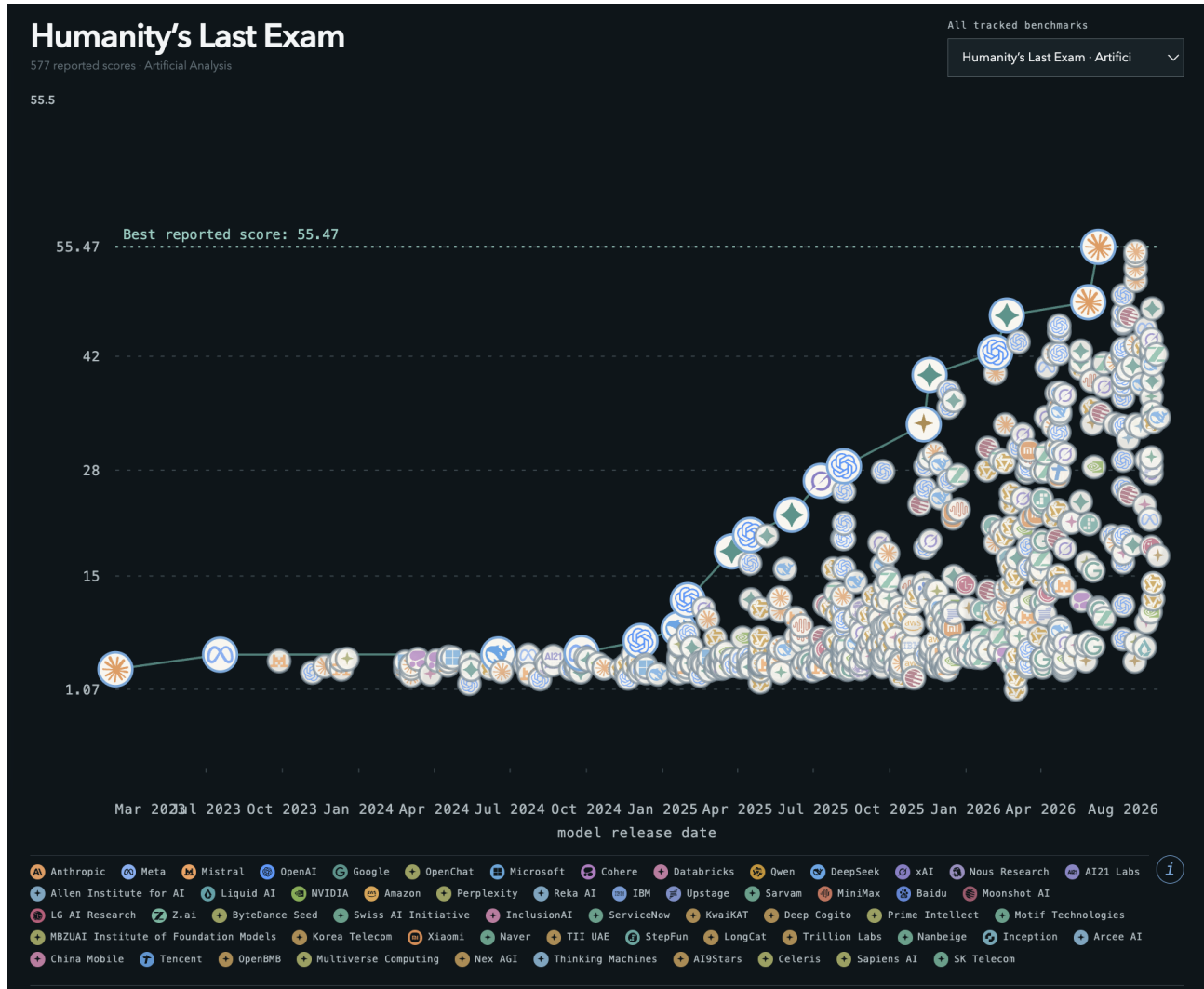
Figure 4: Inspecting Humanity’s Last Exam in Benchmark RADAR. This Artificial Analysis record contains 577 reported scores; the highest displayed score is 55.47. Marks identify model organizations, and the line connects successive best scores ordered by model release date. These are not evaluation dates: older models can be tested after a benchmark’s release. The snapshot illustrates score inspection, without establishing matched evaluation settings or a validated percentage ceiling. Click the image to open the interactive view.
