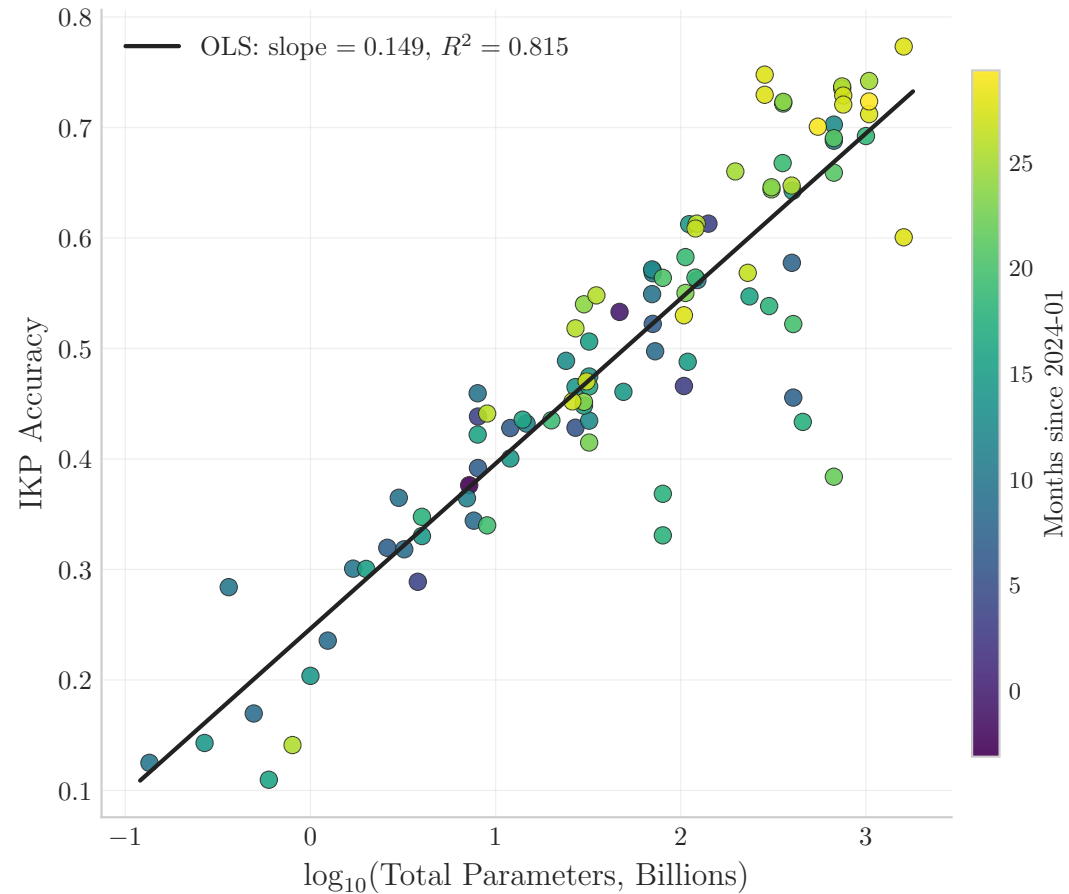
IKP scales with parameters ( n = 100 open models)
