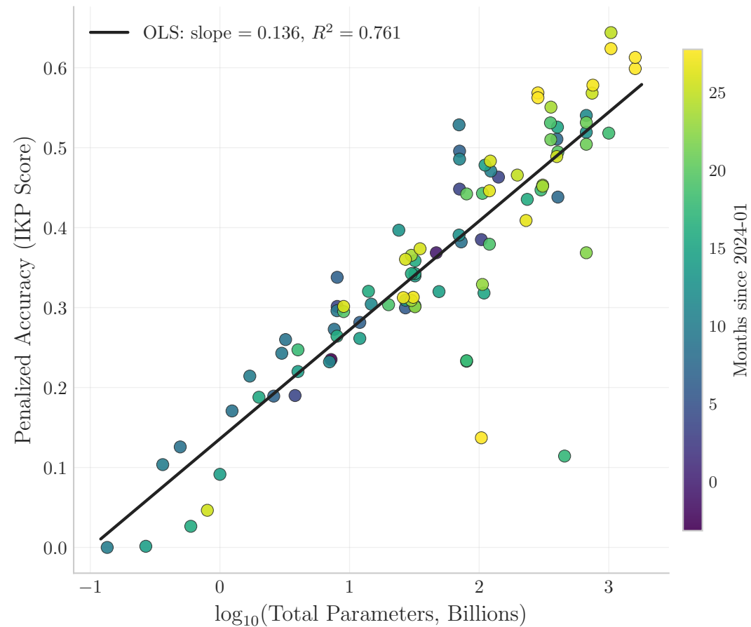
IKP scales with parameters ( n = 96 open models)
