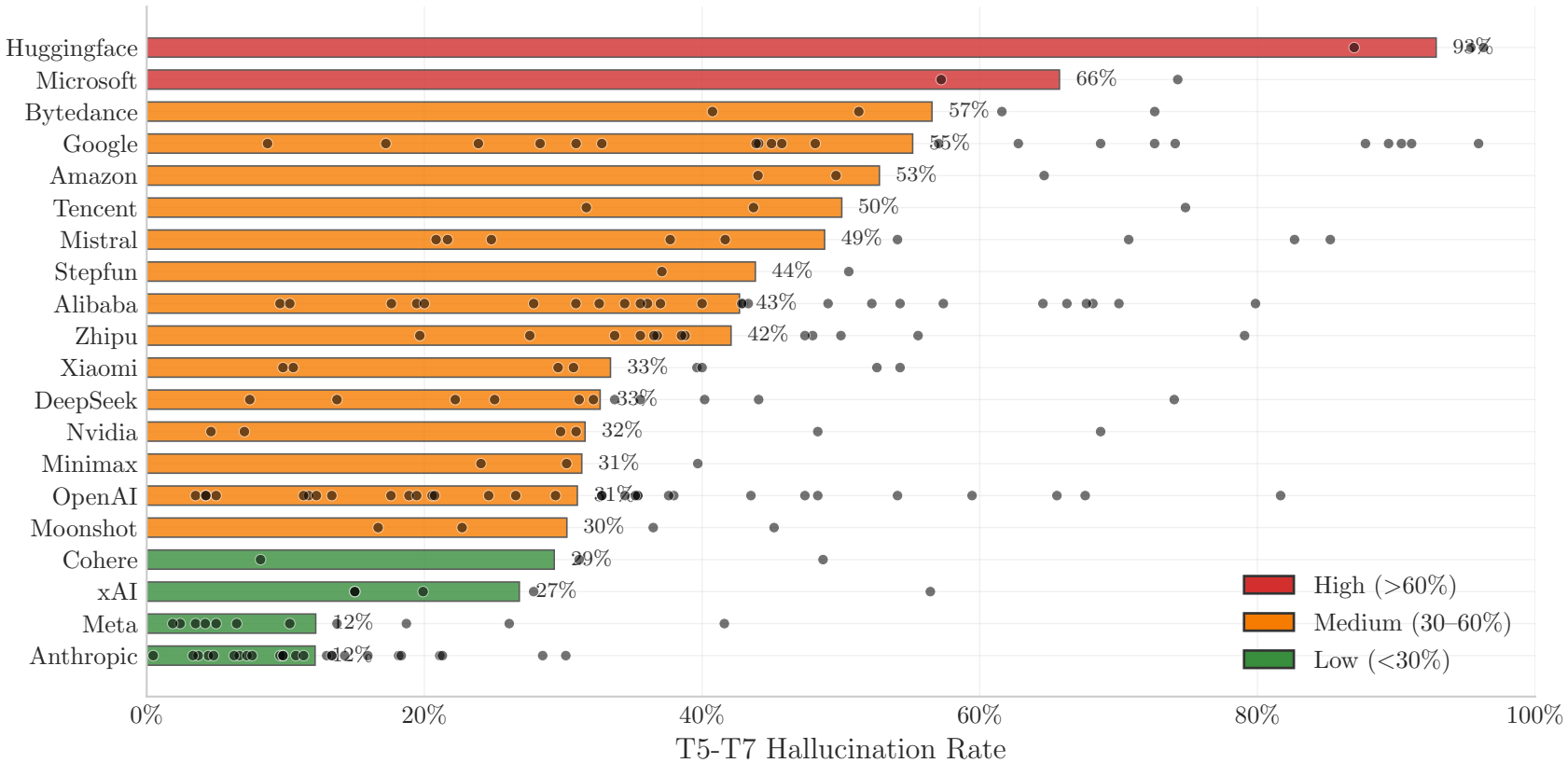
T5-T7 Hallucination Rate by Vendor
