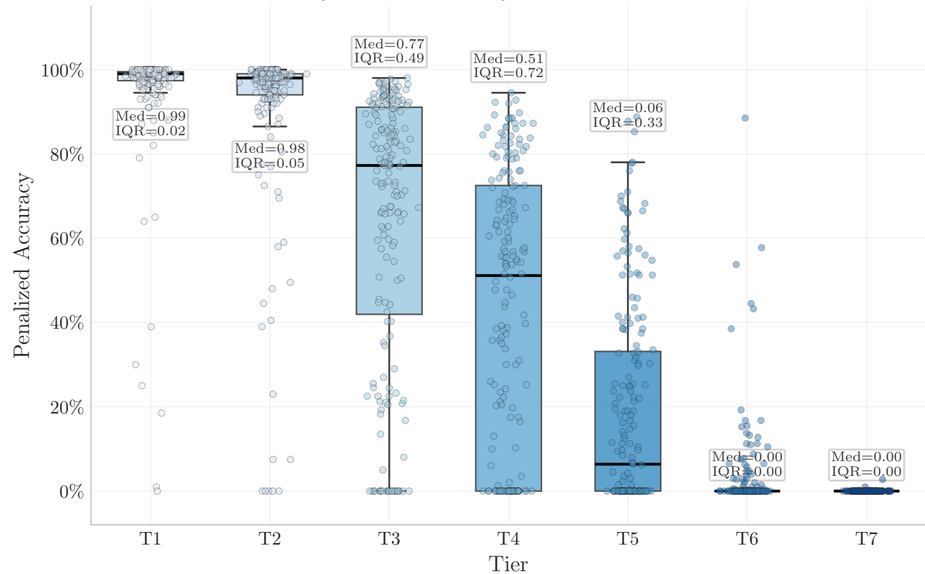
Accuracy Distribution by Tier Across 188 Models
