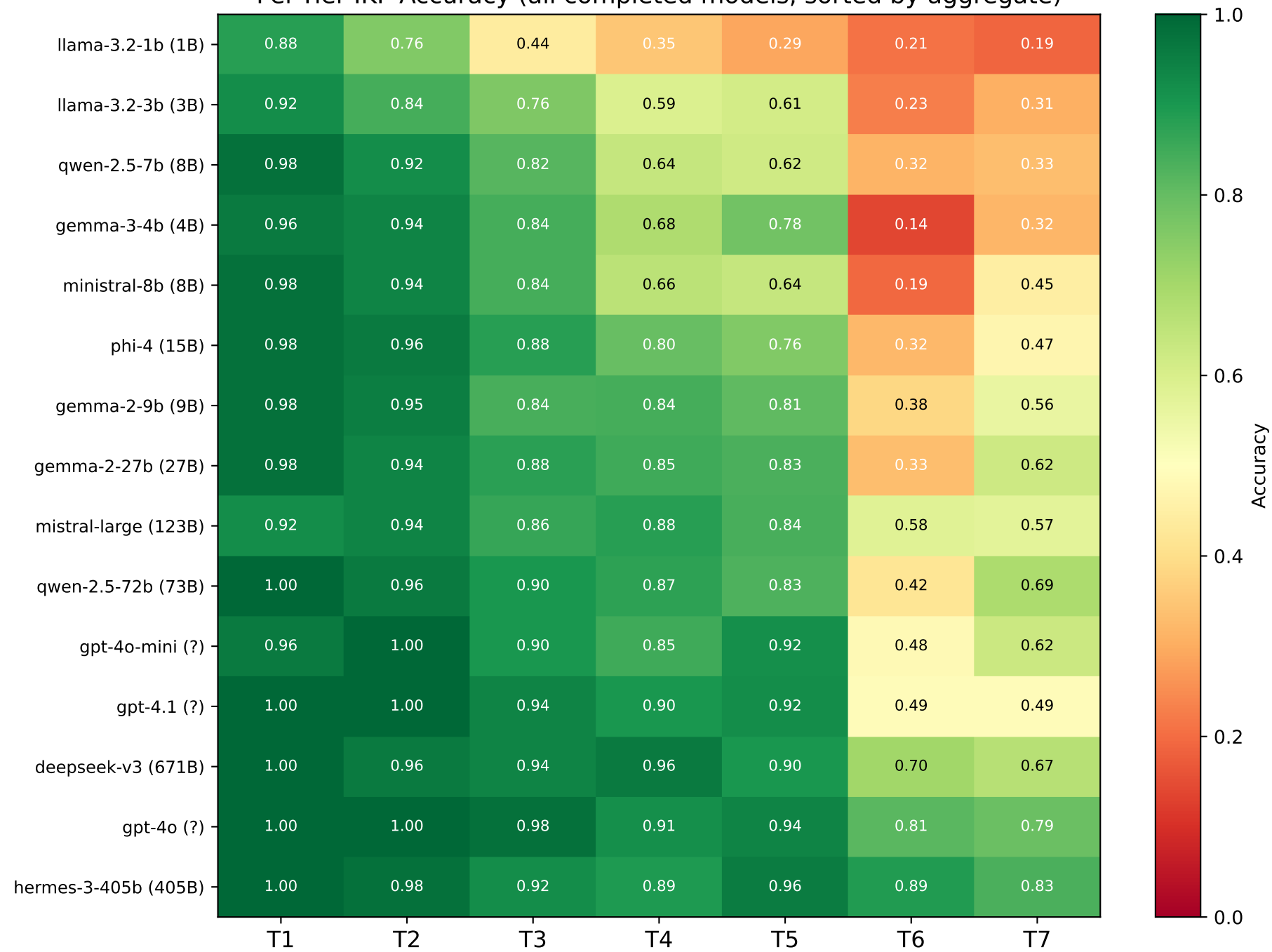
Per-Tier IKP Accuracy (all completed models, sorted by aggregate)
