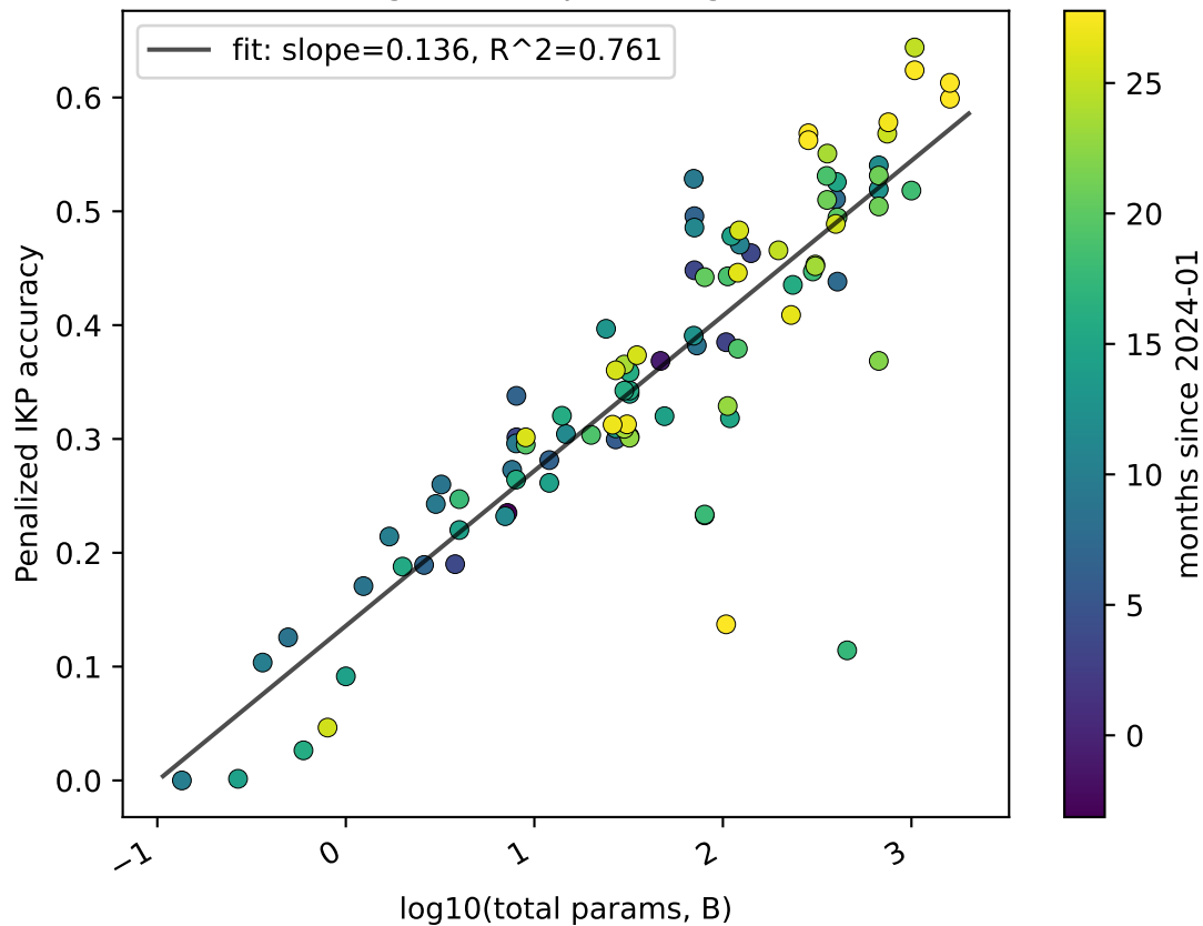
IKP scaling (n=96 open-weight models)
