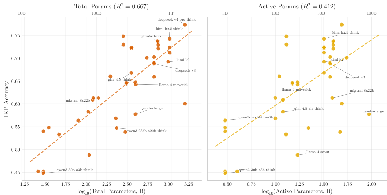
MoE Models: Total vs Active Parameters
