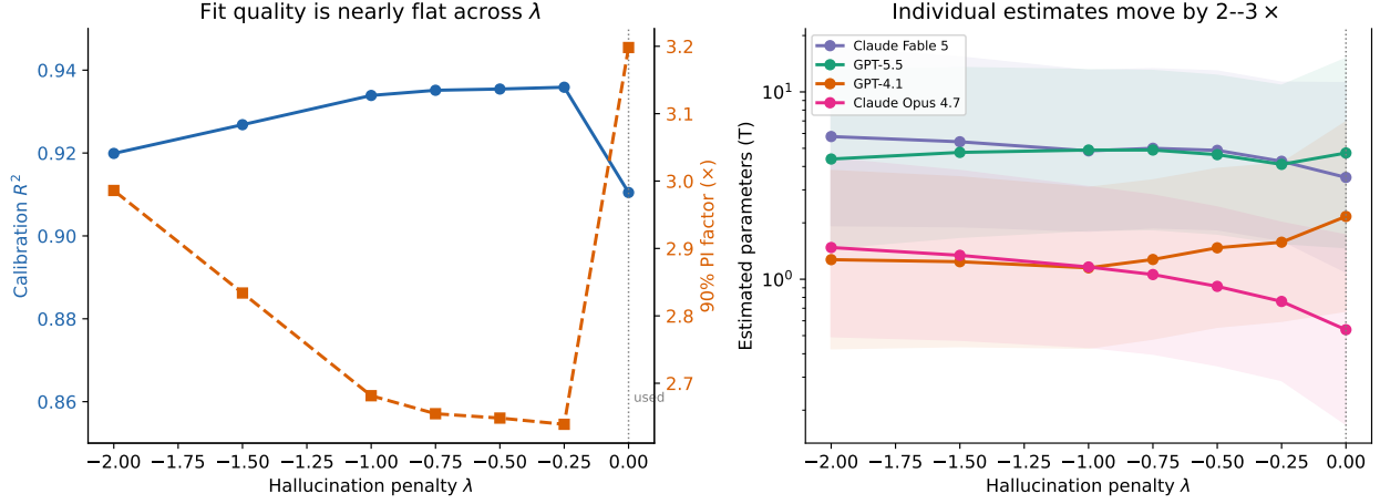
Figure 13: What changes across the hallucination penalty \lambda . Left: calibration fit quality is nearly flat— R^2 stays in [0.91, 0.94] and the 90% prediction-interval factor in [2.6, 3.2]\times (floored scoring for \lambda < 0 ; \lambda = 0 is floor-free). Right: individual frontier estimates (90% bands shaded) move by 2–3 \times and re-order by vendor: as \lambda \rightarrow 0 the confident guesser GPT-4.1 rises while the refusal-heavy Claude Opus 4.7 falls.
