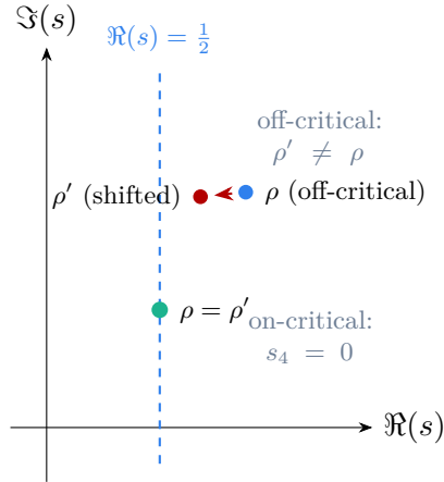
Figure 3. Pole-shift geometry in the complex s -plane. The critical line \Re(s) = \frac{1}{2} is shown dashed. For a hypothetical off-critical zero \rho , the grade-4 contraction maps \rho \mapsto \rho' \neq \rho (red arrow). On the critical line, s_4 = 0 so \rho' = \rho and the shift is trivial (green dot). Compatibility of both grades forces every nontrivial zero into the on-critical case.
