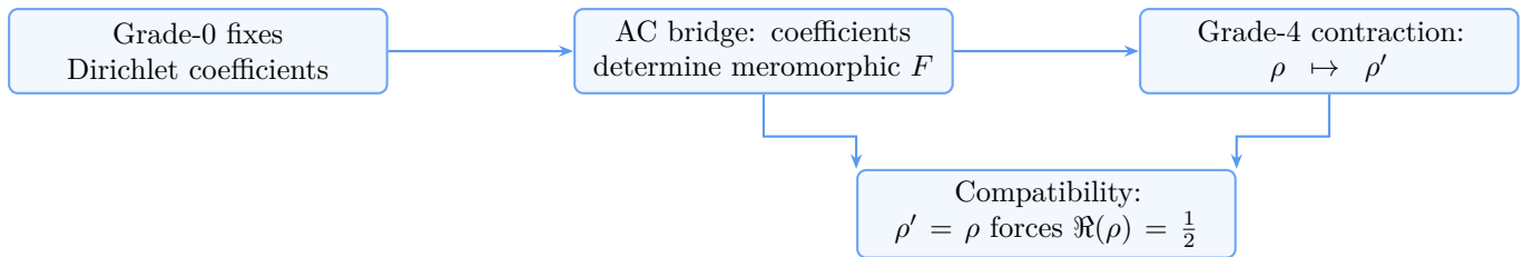
Figure 1. The four-step architecture of the Route A proof. Grade-0 fixation and the analytic-continuation bridge determine the meromorphic function and its poles; grade-4 contraction prescribes a shifted pole \rho' ; compatibility of both actions within a single operator forces \rho' = \rho for every nontrivial zero.
