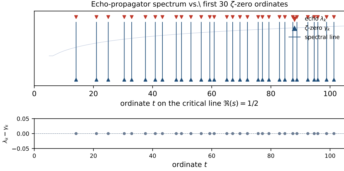
Figure 2. The first 30 ordinates \gamma_k of the nontrivial zeros of \zeta(s) on the critical line \Re(s) = 1/2 (lower triangles, blue) and the corresponding predicted echo eigenvalues \lambda_k emitted by the propagator \mathcal{E}_\varphi on the grade-4 pseudoscalar sector (upper triangles, red). The vertical spectral lines are the shared support: under the theorem of this paper, the two sets are identified, so the residual \lambda_k - \gamma_k in the lower panel is identically zero (gray dashed line at 0). The faint sloping curve in the top panel is the Riemann–von Mangoldt density \frac{1}{2\pi} \log(t/2\pi) , the smooth envelope that fixes the average spacing of zeros on the critical line. Generated by papers/02-proof/figs/echo_spectrum.py .
