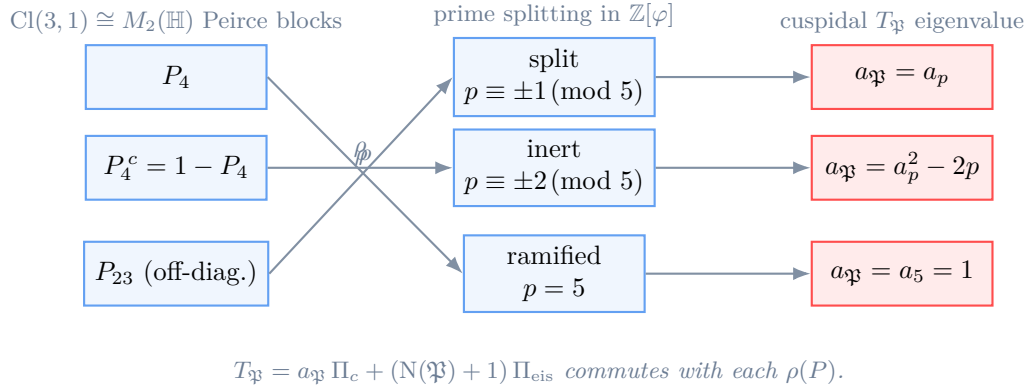
Figure 2. The Peirce–prime-splitting bridge for the homomorphism \rho : \text{Cl}(3, 1) \rightarrow \text{End}(H_1) of Paper VI. The three Peirce blocks of M_2(\mathbb{H}) = \text{Cl}(3, 1) – the boundary idempotent P_4 , its complement P_4^c , and the off-diagonal P_{23} block – map under \rho to the three splitting types of rational primes in \mathbb{Z}[\varphi] . The Hecke operator T_{\mathfrak{p}} commutes with each Peirce projector and acts on the cuspidal summand \Pi_c with the splitting-type-stratified eigenvalues (a_p, a_p^2 - 2p, 1) shown at right. This is the algebraic content of the entire Paper VI in one picture: which prime splitting type a prime belongs to is the same data as which Peirce block of \text{Cl}(3, 1) it factors through.
