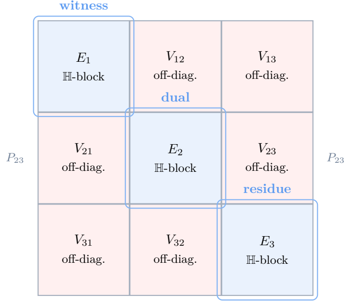
J_3(\mathbb{O}') Peirce block structure: diagonal \cong \mathbb{H} (idempotents E_i ), off-diagonal \cong \mathbb{O}' (octets V_{ij} )
