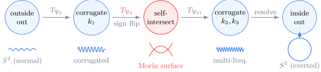
Figure 1. Schematic of sphere eversion realized as Hecke propagation. The five stages correspond to: (1) the initial sphere with outward normal; (2) corrugation at frequency k_{\mathfrak{P}_5} = 5 (ramified prime); (3) the Morin-type self-intersection where the cuspidal sign flips ( a_{\mathfrak{P}_3} = -5 , inert prime); (4) multi-frequency corrugation after the split prime \mathfrak{P}_{31} ; (5) the everted sphere with reversed orientation. Each arrow is a single Hecke step \psi_k = T_{\mathfrak{P}_k} \psi_{k-1} . The sign flip at stage 3 is the arithmetic realization of Thurston’s topological eversion.
