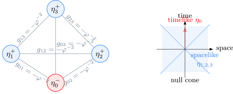
Figure 2. The four golden-coupled null generators of the depth-2 substrate form a regular tetrahedron with every pair coupled at the identical strength g_{ij} = -\varphi^{-2} . Diagonalising the Gram matrix produces three positive eigenvalues +\varphi^{-2} (corresponding to the spacelike children \eta_{1,2,3} ) and one negative eigenvalue -3\varphi^{-2} (the timelike seam \eta_0 ), fixing the \text{Cl}(3,1) convention (+, +, +, -) . Inset: the null cone defined by \langle V \cdot V \rangle_0 = 0 separates the spacelike children (blue, \langle V \cdot V \rangle_0 > 0 ) from the timelike seam (red, \langle V \cdot V \rangle_0 < 0 ); the framework’s content register lives in the spacelike interior, the seam (context) on the timelike axis.
