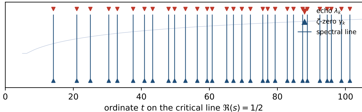
Echo-propagator spectrum vs. first 30 \zeta -zero ordinates
