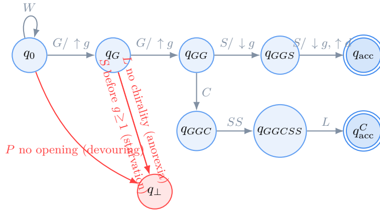
(Path through 5 of the 64 FST states; \Sigma = \{W, G, S, C, L, P, X\} .)
