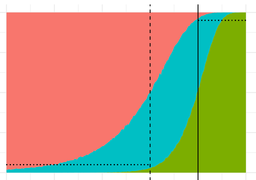
D: Hypothesis testing with T_l = 86.2\% T_u = 96.2\%
