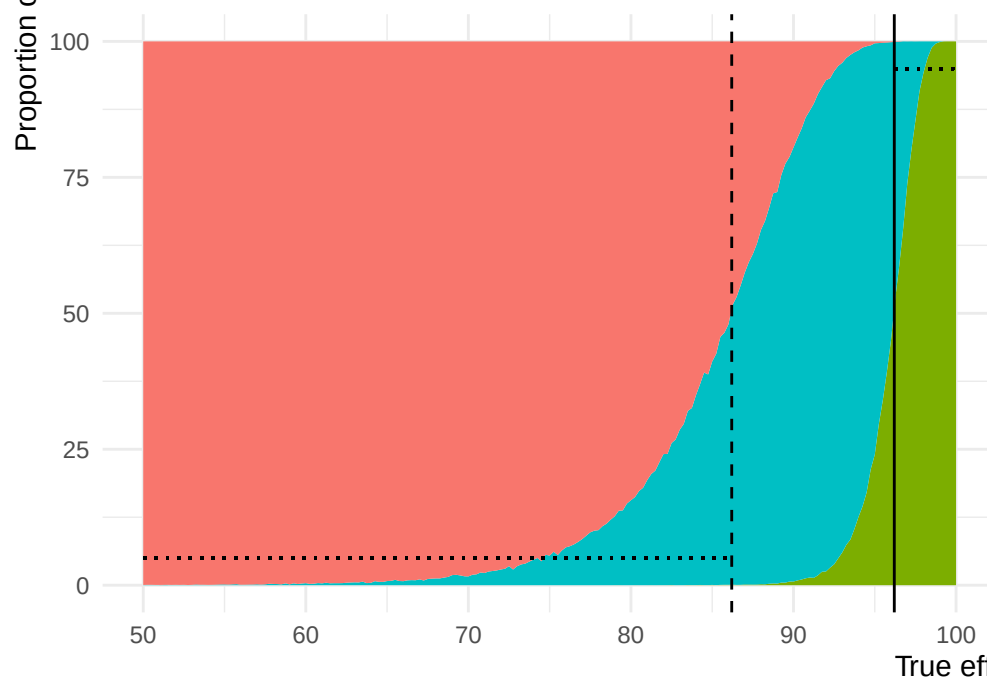
C: Point estimate with T_l = 86.2\% T_u = 96.2\%
