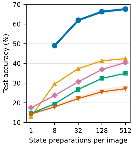
(b) CIFAR-10
