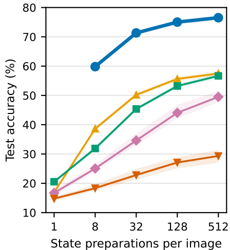
(a) Fashion-MNIST
