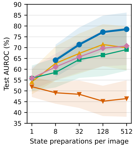
(c) BreastMNIST
