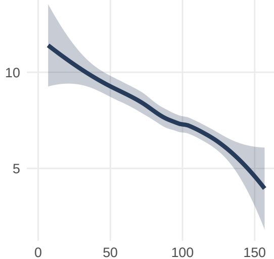
SOFA Score
