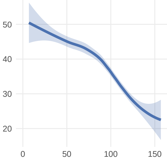
SAPS Score
