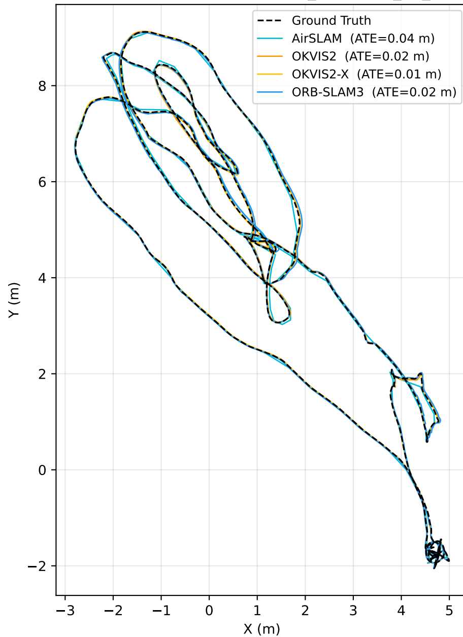
Trajectory comparison — euroc_mav / MH_01_easy
