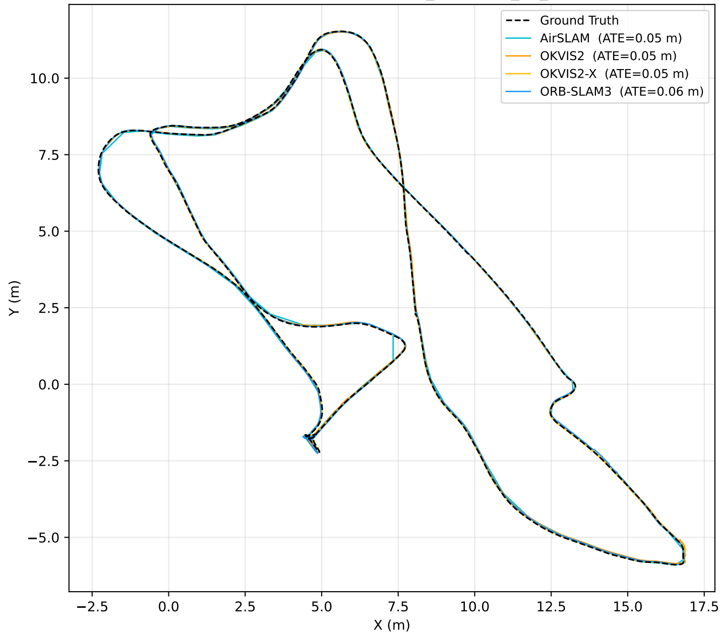
Trajectory comparison — euroc_mav / MH_05_difficult
