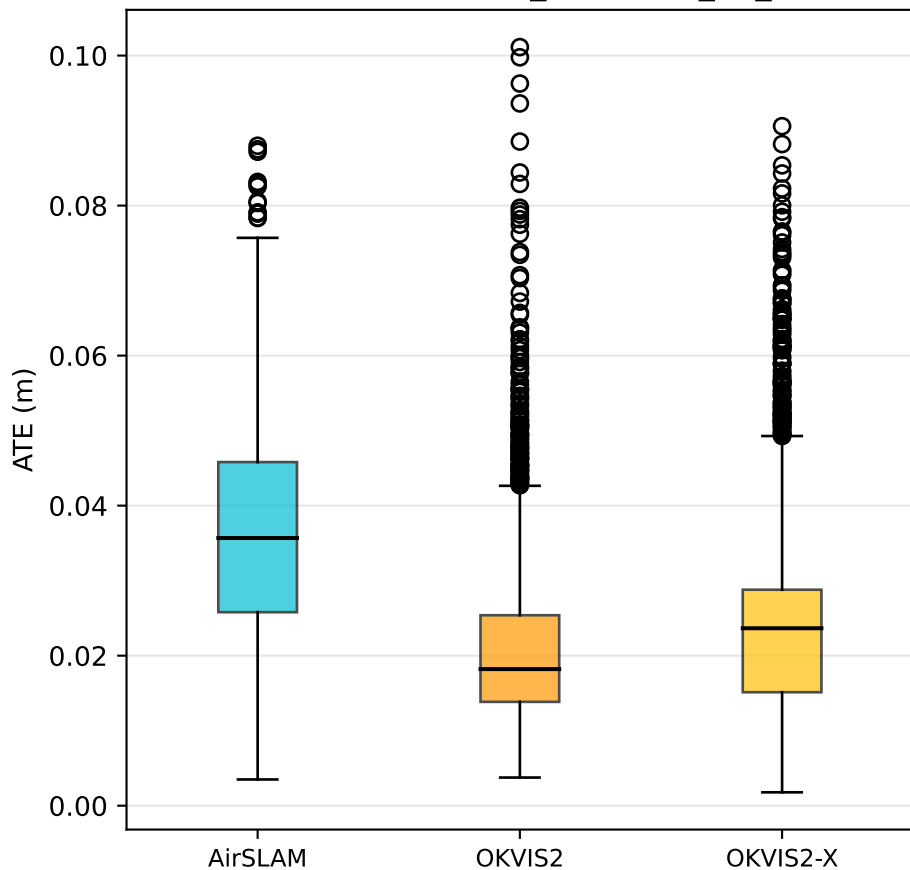
ATE distribution — euroc_mav / MH_03_medium
