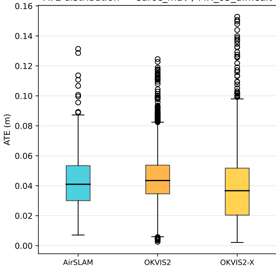
ATE distribution — euroc_mav / MH_05_difficult
