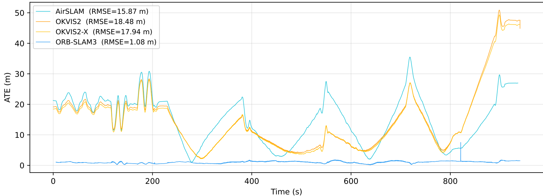
ATE over time — rosariov2 / sequence1
