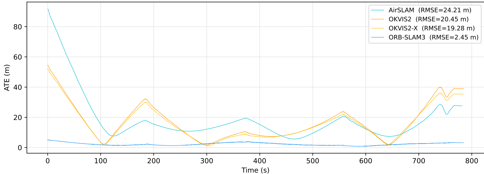
ATE over time — rosariov2 / sequence5
