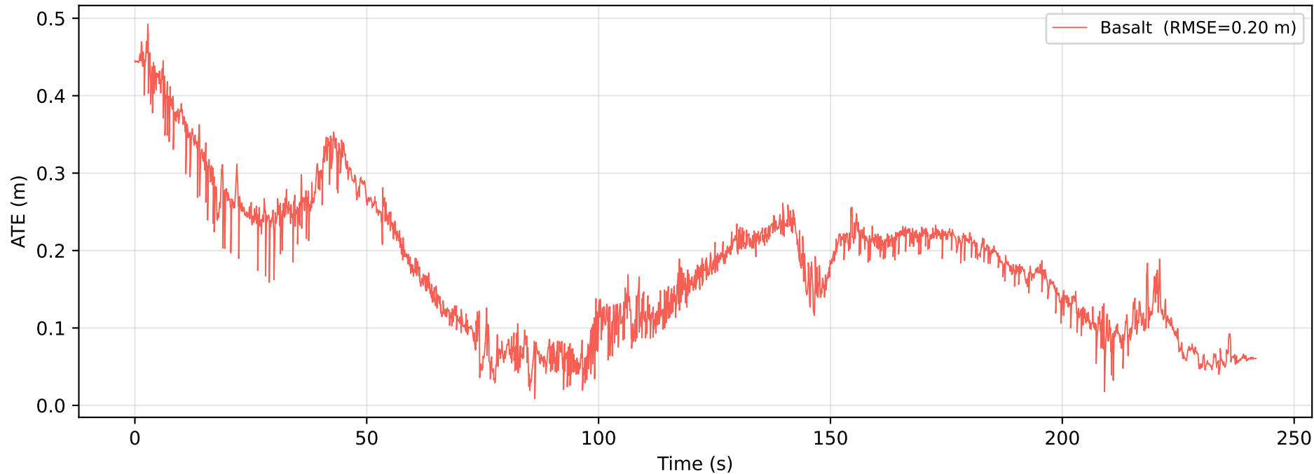
ATE over time — hortimulti / strawberry03
