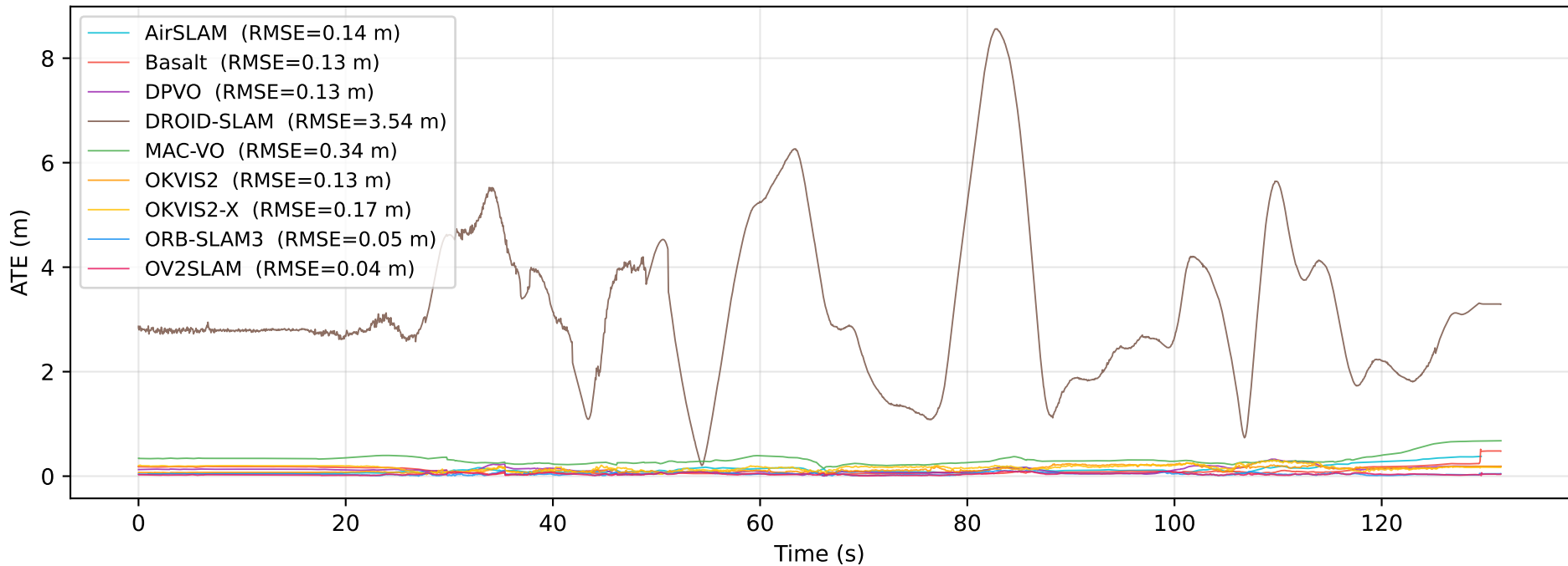
ATE over time — euroc_mav / MH_03_medium
