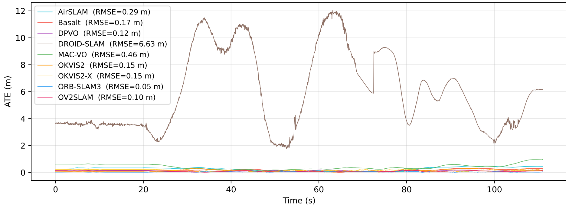
ATE over time — euroc_mav / MH_05_difficult
