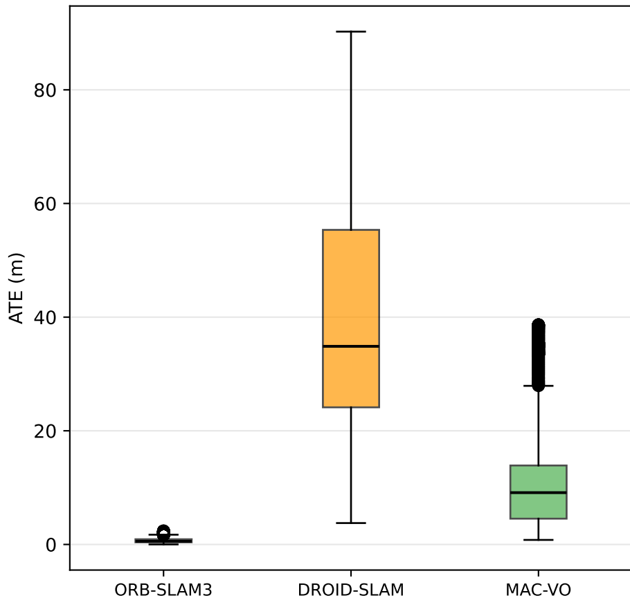
ATE distribution — rosariov2 / sequence1
