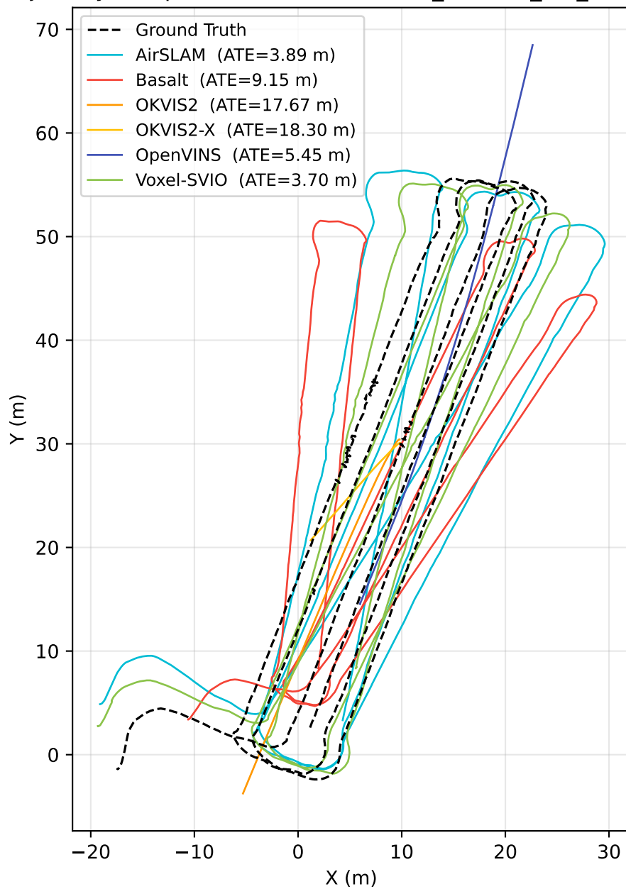
Trajectory comparison — zed2i / field1_110426_full_10fps_q90
