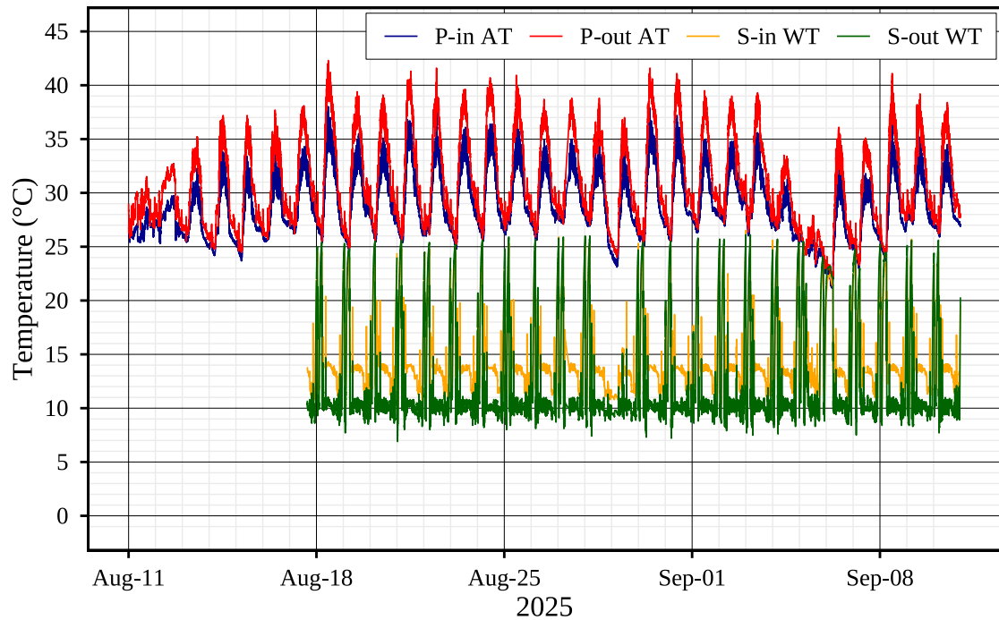
Average temperature of 2 outdoor units
