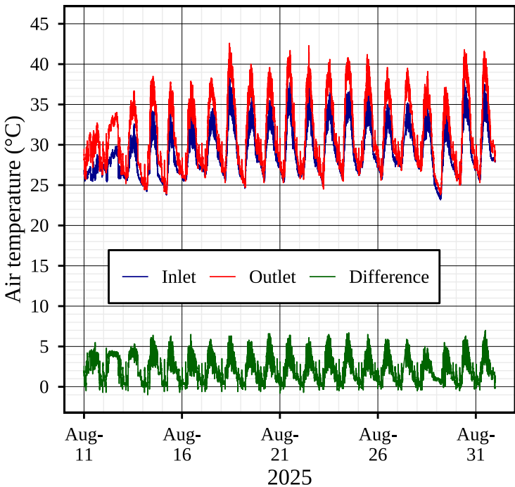
Temperature of 1st outdoor unit
