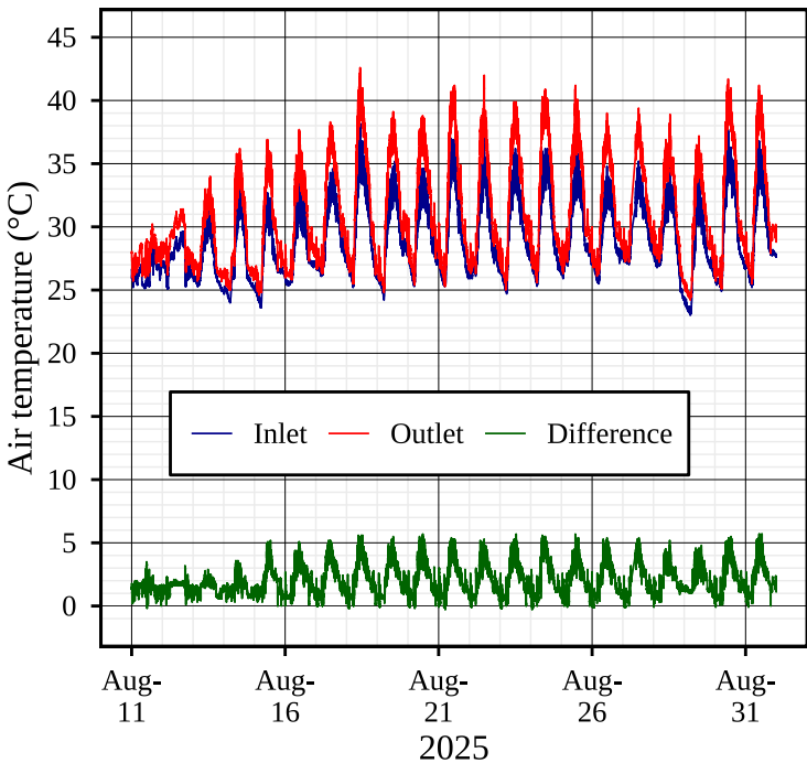
Temperature of 2nd outdoor unit
