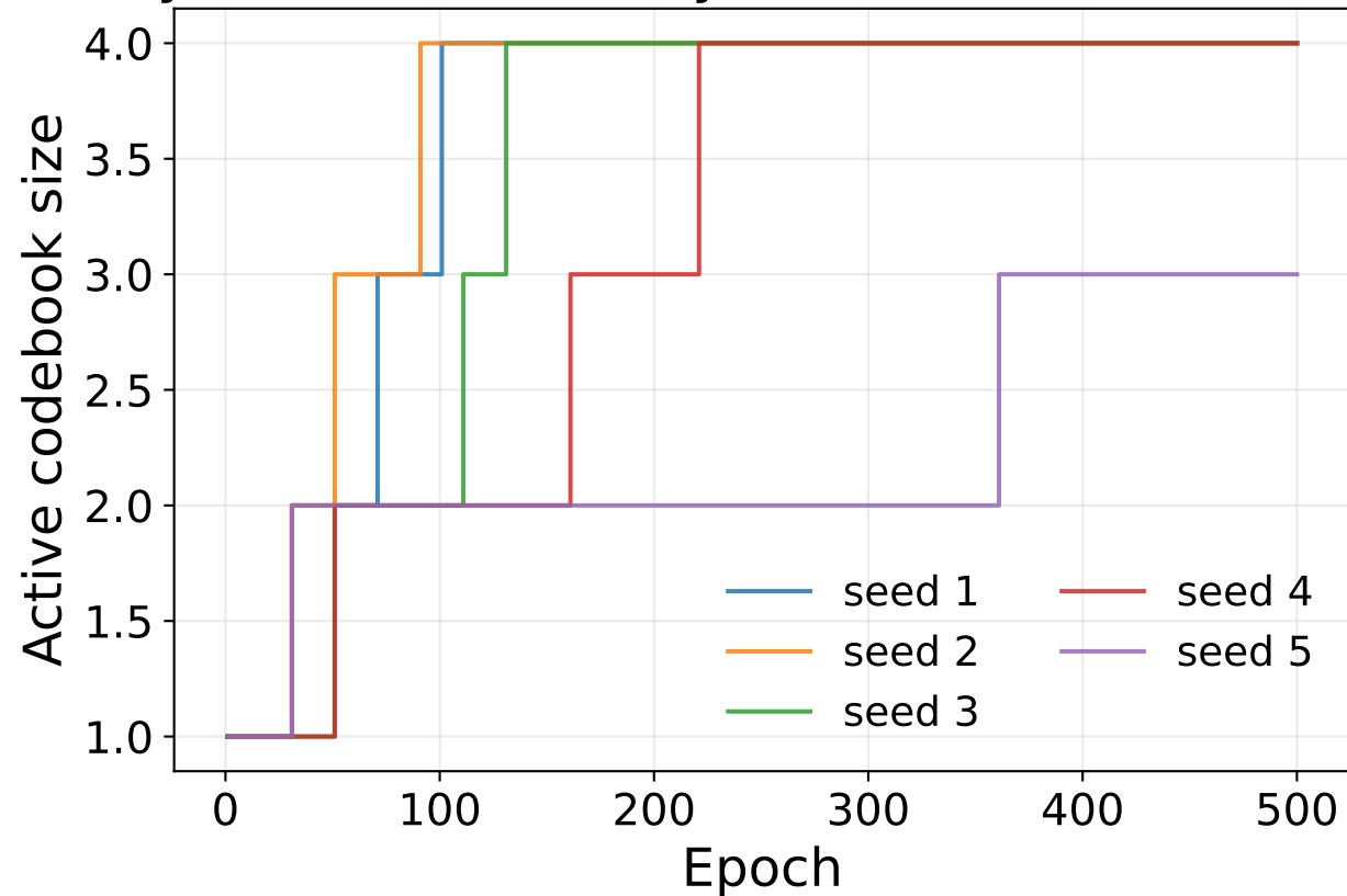
Dynamic VQ stability across seeds — level 1
