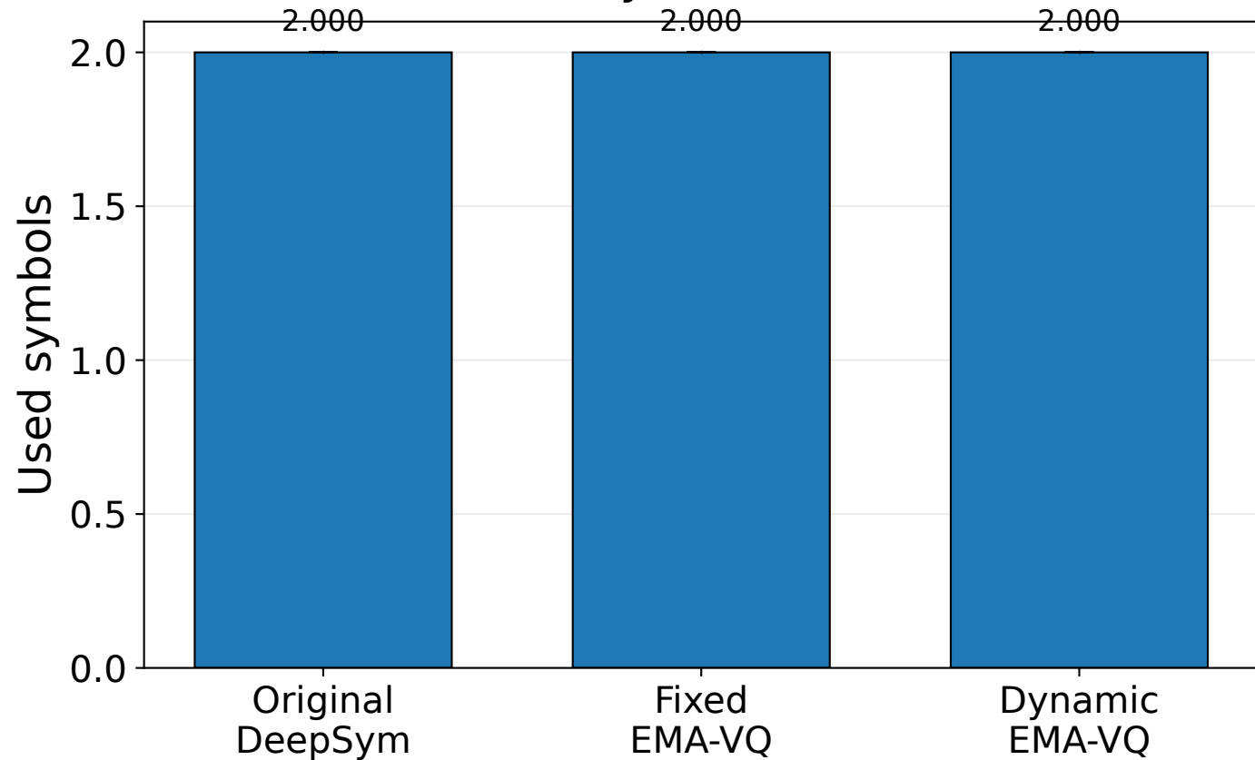
Relation-symbol utilization
