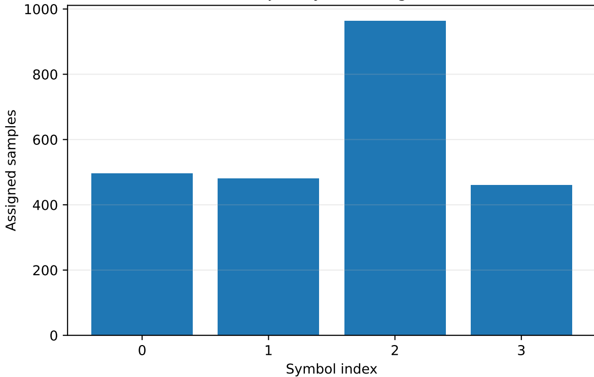
Object-symbol usage
