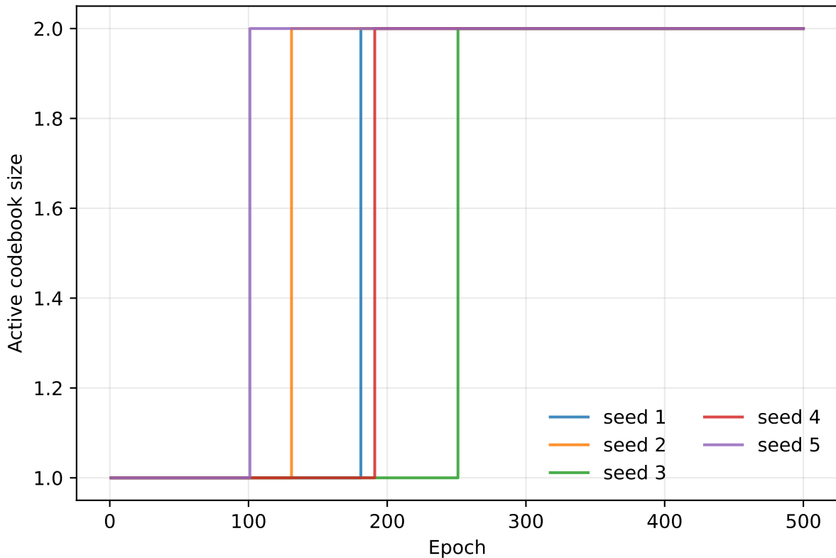
Dynamic VQ stability across seeds — level 2
