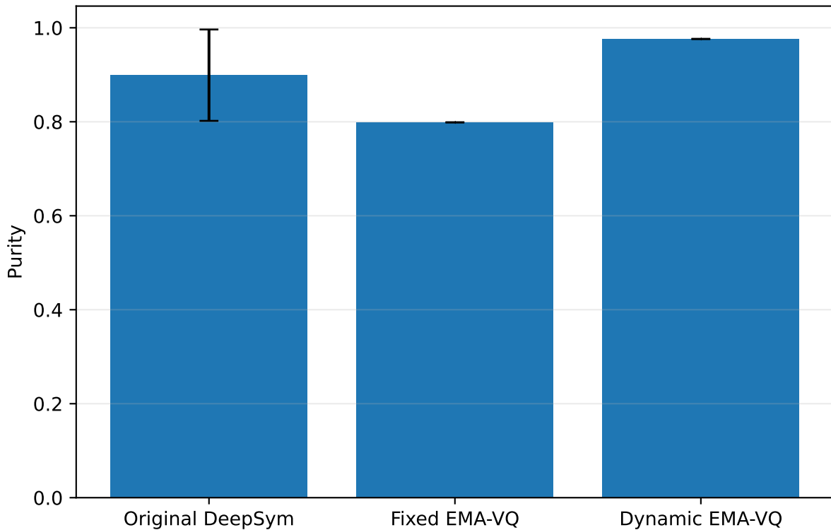
Affordance-relevant object-symbol purity
