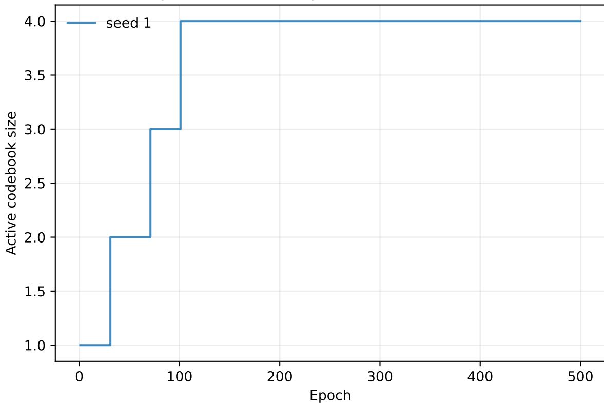
Dynamic VQ stability across seeds — level 1
