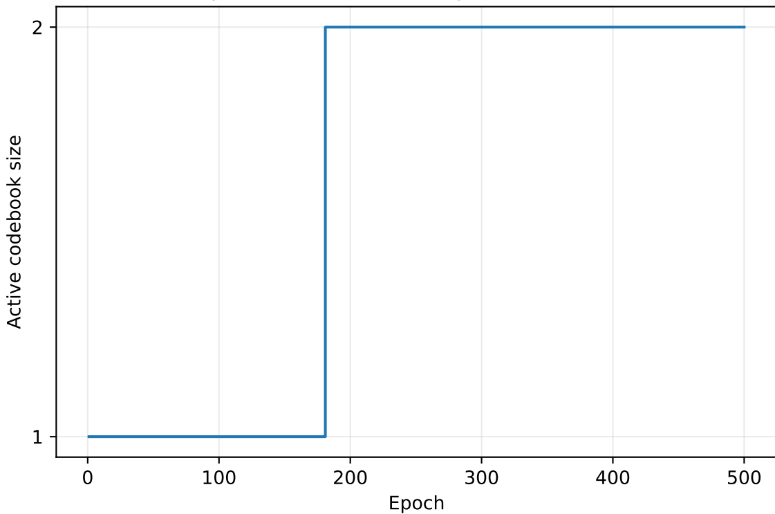
Dynamic VQ codebook growth — level 2
