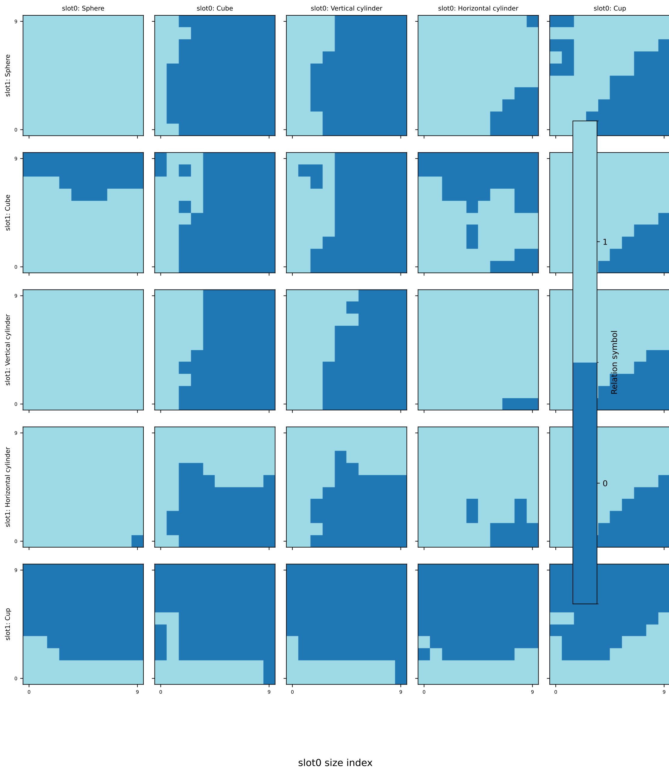
Learned relational symbol by ordered object pair and size x: slot0 size, y: slot1 size
