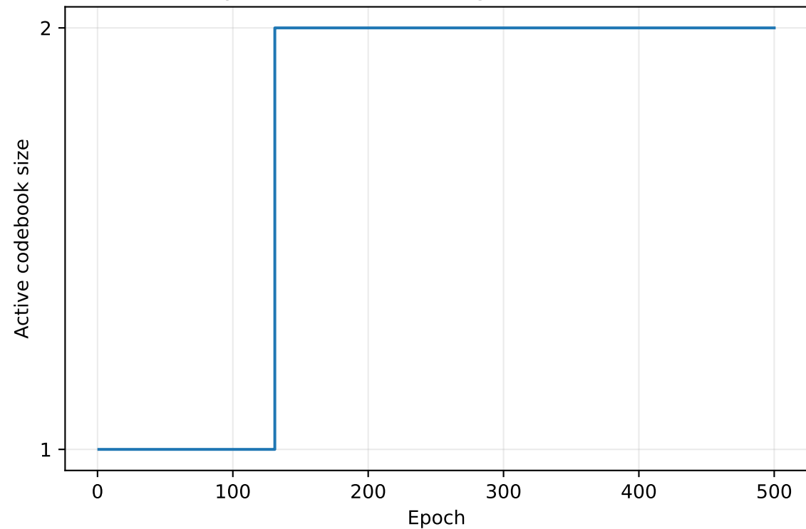
Dynamic VQ codebook growth — level 2
