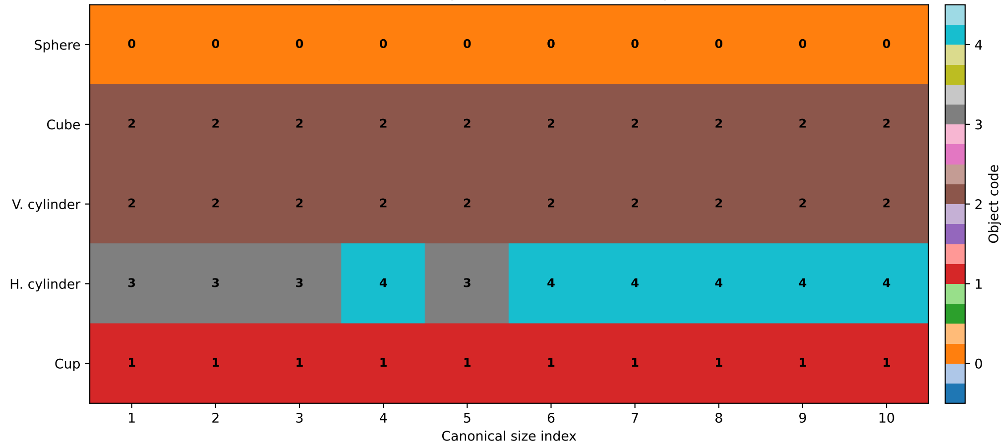
Object-code assignment on 50 canonical objects
