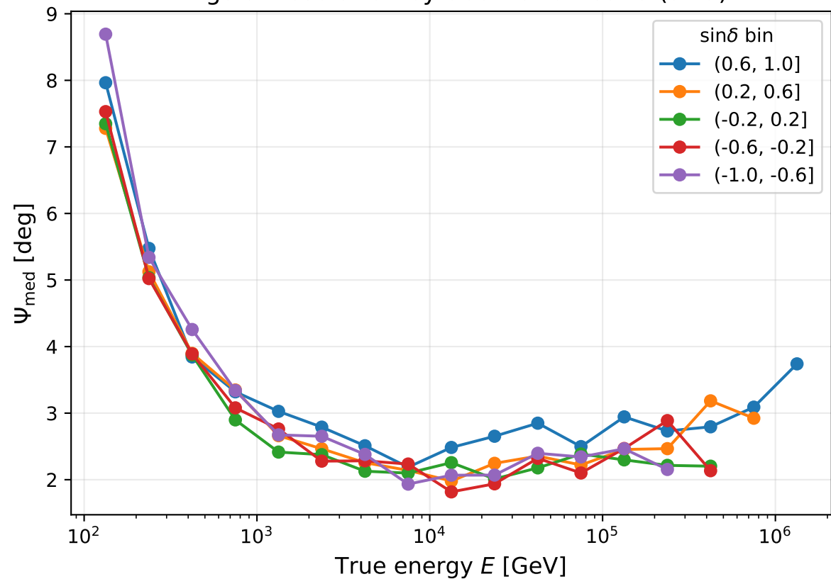
Angular resolution by declination band ( \sin\delta )
