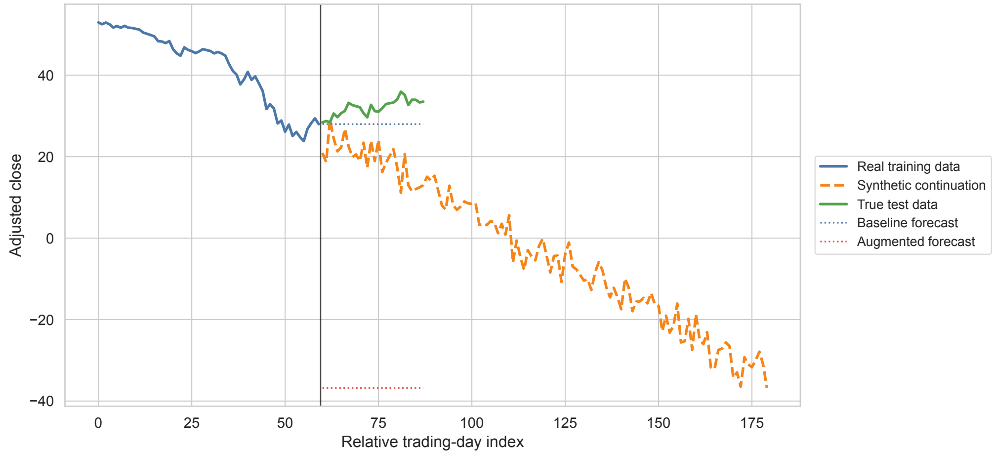
XOM_w12_s0000: naive, ratio=2.0, MAPE diff=202.84
