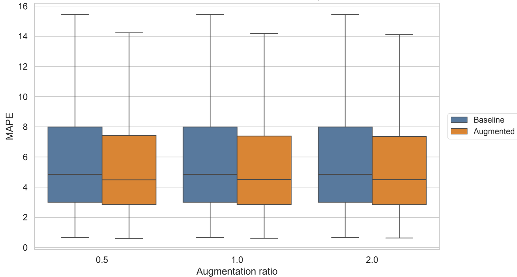
Distributional Shift in MAPE After Statistical Augmentation
