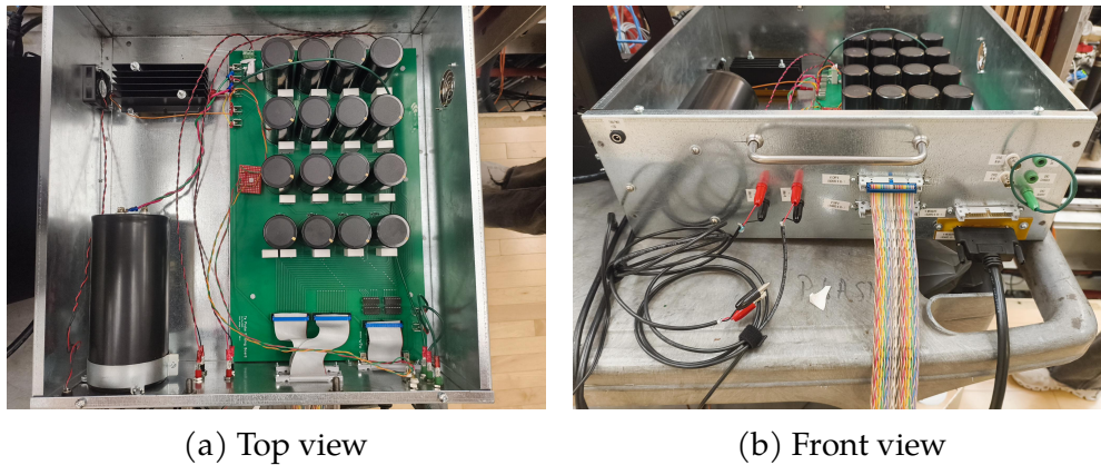
Figure 3.8: An image of the circuitry for the new bias power supply. In panel ???: the top left is a fan for cooling the charging resistor hidden beneath a heat sink in black, the bottom left shows the negative capacitor that sets the ground of the rest of the circuit, the top right black cylinders are the individual tip capacitors and white rectangles are high power resistors for the voltage division, bottom right are connections to the front panel. In panel ???: the top left is the fan power, the red and black banana connections are to the power supplies, the rainbow ribbon cable is the connection to send bias to the tip circuit, the bottom right black cable is for measurement of the bias voltage, and the green banana is a connection to the laboratory ground.
