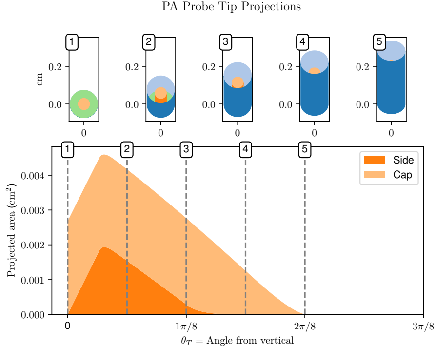
Figure 4.16: The bottom plot shows the projected area of the core as a function of direction. The top plots are what the probe tip looks like from specific direction associated with the vertical dashed grey lines. The shell is blue, insulation green, and core orange.
