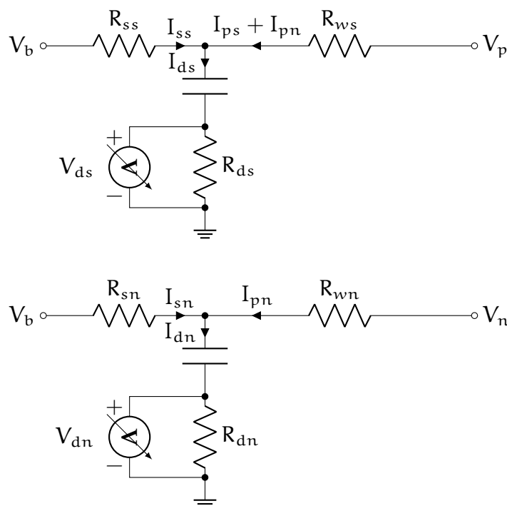
Figure 3.10: Circuit for a single tip on the Langmuir probe alongside the circuit for measuring noise. The V_b inputs are the same for both circuits but since the bias not change during a shot we will ignore any currents flowing between the circuits. The subscripts are organized as (element, circuit) where the elements are b = \text{bias} , s = \text{sense resistor} , w = \text{wire} , p = \text{probe} , d = \text{digitizer} and the circuits are n = \text{noise} , s = \text{signal} . In our equations we don't use the raw voltages from the digitizers ( V_{ds} and V_{dn} ) and instead use the currents ( I_{ds} and I_{dn} ) which we can find using V = IR .
