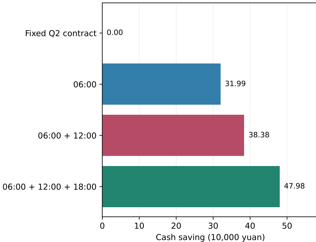
Q3: value of prespecified intraday release schedules (settlement A)
