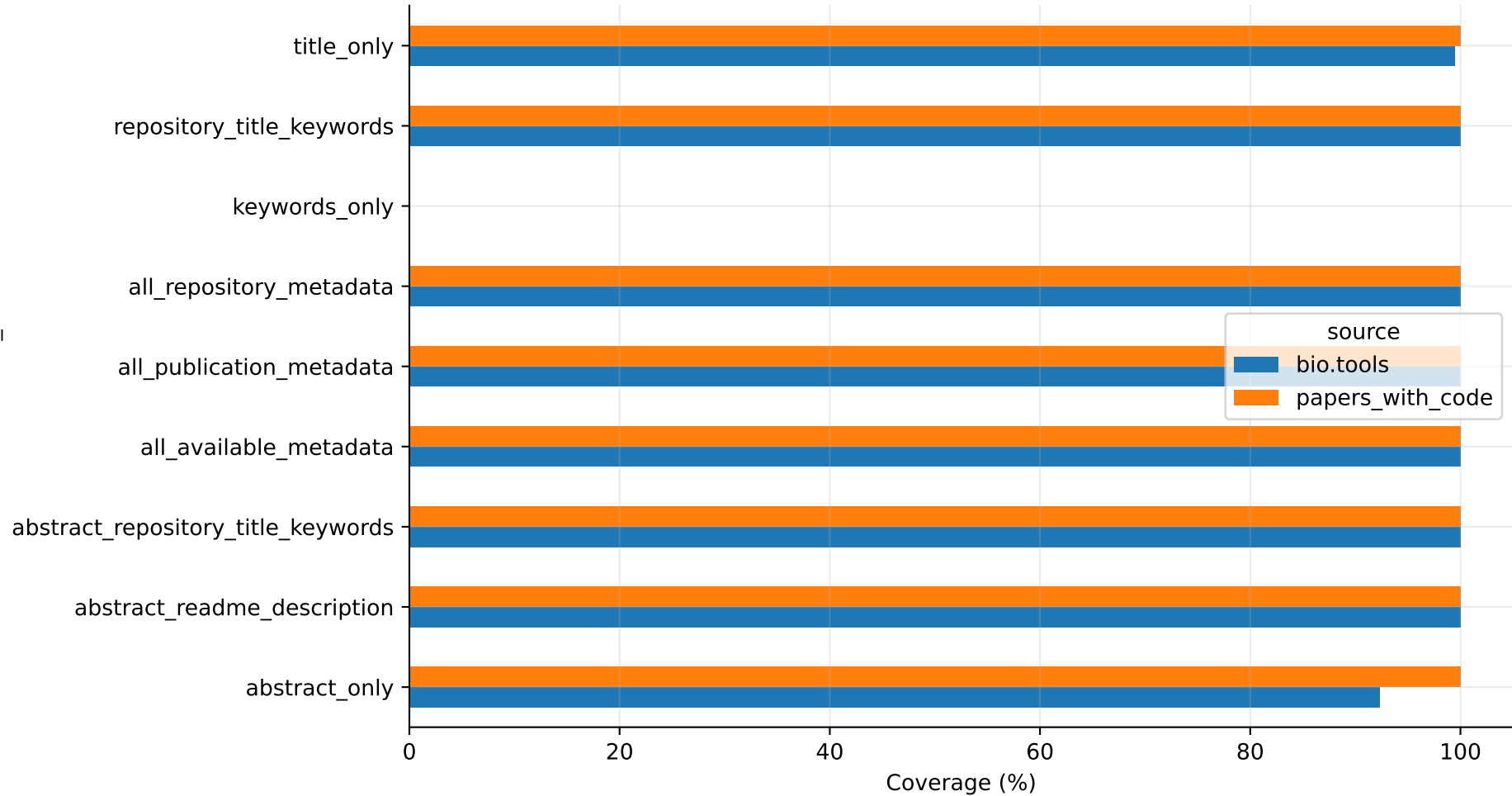
Attribute Coverage
